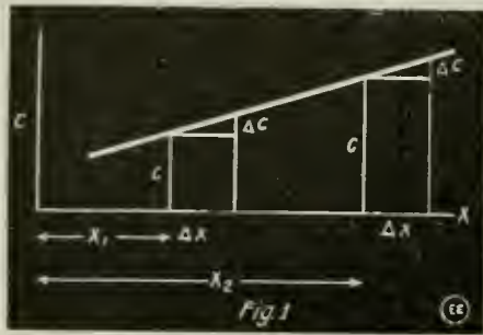
The Shape of the Ordinary Variable Condenser Moving Plate is Such That for Equal Angular Displacements From the Position of Minimum to That of Maximum Capacity, an Approximately Straight Line Variation of Capacity is Obtained.
