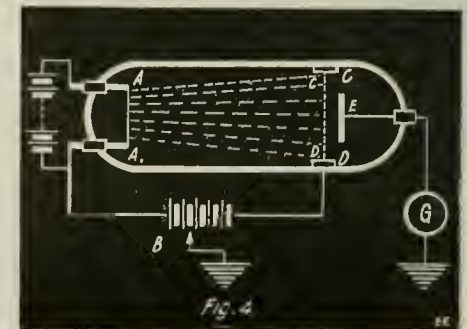
Design of Vacuum Tube Used by Franck and Hertz in Their Researches on the Conduction of Electricity Thru Gases.
