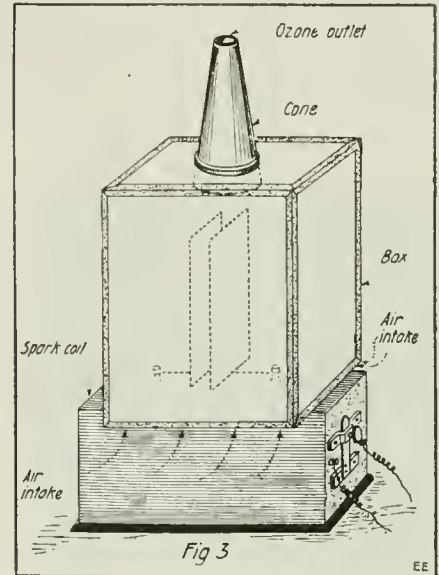
Another Form of Ozone-Concentration Cabinet Made to Fit on Top of the Spark Coil. Air Intake Vents Are Provided in the Bottom of the Enclosure.
