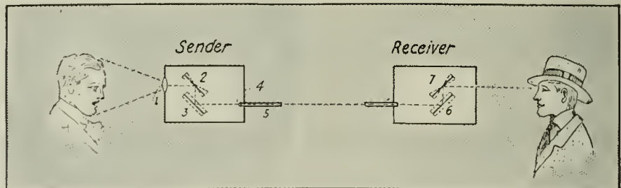
Fig. 5 Depicts the Sinding-Larsen Telephot. Two Mirrors Vibrating at Different Frequencies Cut Up the Light Rays. These Light Rays Are Past Thru a Metallic Tube Having Strong Reflecting Inner Surfaces. At the Receiver, the Light Rays Arer Past Thru a Similar System as the Sender and the Picture Is Thus Reconstructed.
