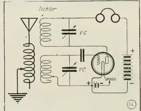
Simple Form of "Tickler Circuit" for Audion Which Gives Highly Selective Tuning, as Practical Experience Demonstrates.
