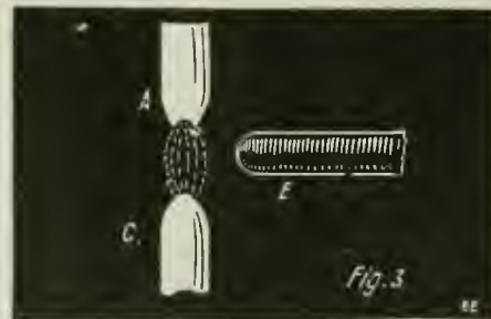
Dr. J. A. Fleming Explored the Electric Arc With an Auxiliary Pole E, and Found That While the Arc Was Burning He Could Get a Current Between E and C, But Not Between A and E, Keeping E Cold.
