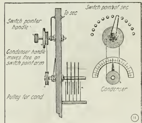
Here's a Good Method of Simplifying the Tuning of a Radio Condenser and Inductance. The Shaft Is Belted or Geared to the Inductance. The Condenser Shaft Is Belted or Geared to the Inductance Switch Handle.
