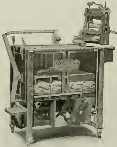
A New Electrically Driven Washing Machine that Operates on the Vacuum Principle. There Are no Pegs or Drums to Catch and Tear the Clothes—Even the Finest Fabrics Can Be Washed in It. It Has a Motor-Operated Wringer.
