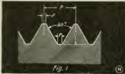
This Shows the Shape and Formation of the U. S. Standard Machine Screw Thread. Note the Flat Edge and Bottom.
