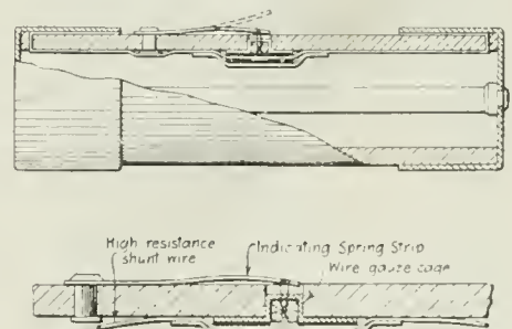
Something Every Electrical Maintenance Man Will Appreciate—a "Tell-Tale" Fuse Blowout. When the Fuse Blows the Indicator Spring Is Released As Noted.
