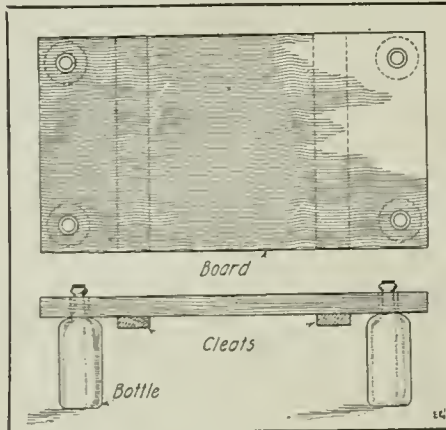
Efficient Static and High Frequency Insulating Stool.
