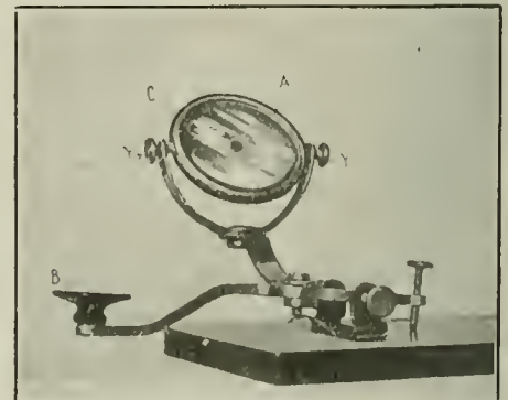
A Simply Made "Heliograph" Similar to That Used by Army Signal Corps. It Will Prove Very Effective for "Boy Scout" Signaling Work.
