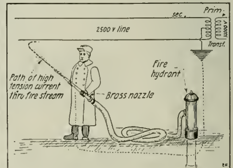
Diagram Showing How a Fireman Can Receive An Electric Shock Thru a Stream of Water From a Fire Hose.
