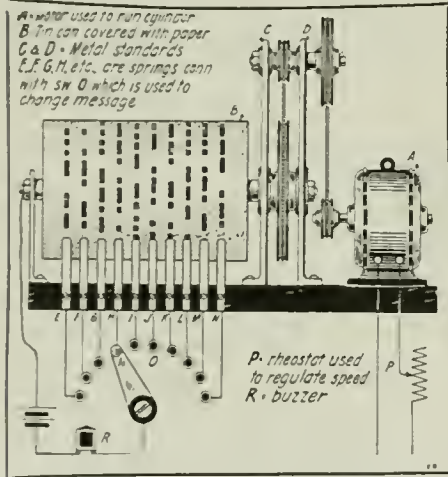
With This Home-Made "Omnigraph" You Have Available a Wide Variety of Radio Signals Which Can Be Changed Instantly by Moving a Switch.
