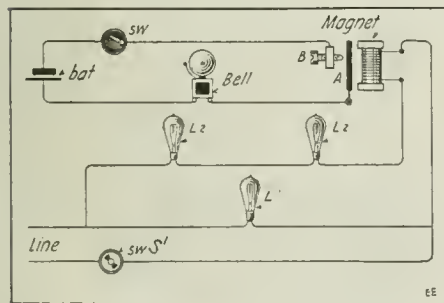
Clever Lamp and Bell Circuit Alarm Successfully Used to Catch "Copper Thieves," Who Cut the Line and Attempted to Depart Hence With a Goodly Length of It.
