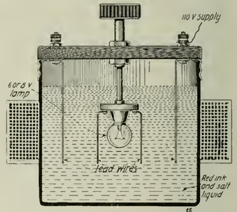
A Somewhat Different Electric Dark-Room Lamp for the Photographer. It Is Used on a 110 Volt Circuit in Series With a 110 Volt, 16 C.P. or 20 Watt Lamp. The Battery Lamp Should Be Thoroly Water-Proofed.
